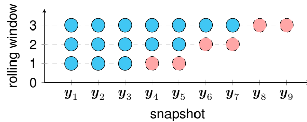
Figure 5 Graphical scheme of the rolling forecasting on traffic states. The snapshot y_t \in \mathbb{R}^N, \forall t \in \{1, \dots, T\} refers to the t -th column of \mathbf{Y} \in \mathbb{R}^{N \times T} .
